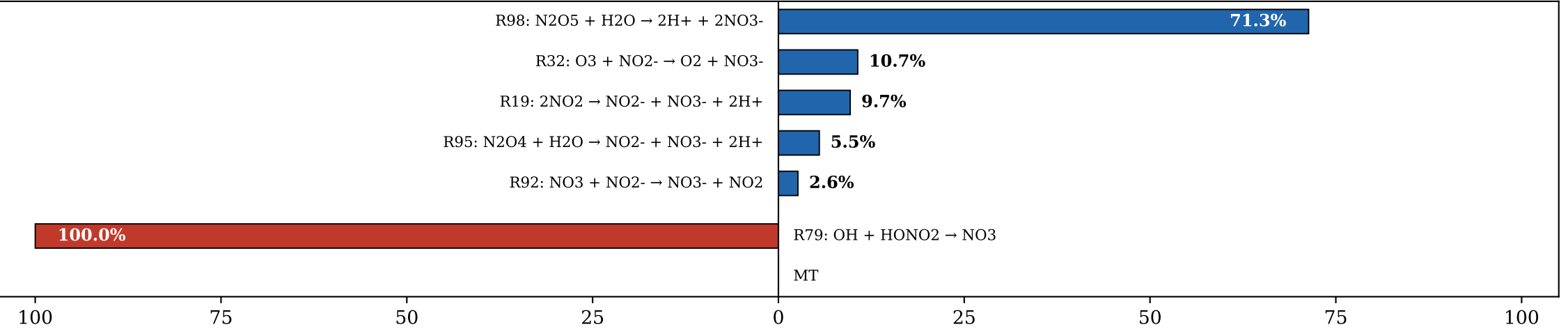
(b) O 3 (Σsrc = 1.47e-08 M/s)
